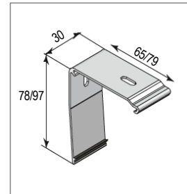
S2/S3 bracket, on wall or in ceiling.
