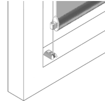
Wired side guiding
