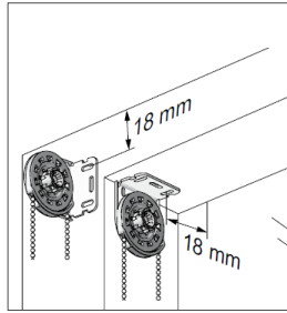
Mounting options: on face wall, in ceiling or in the side of the recess.
