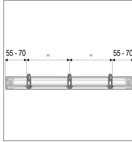
Distance between brackets.
