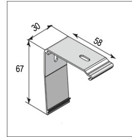
Bracket, on wall or in ceiling.
