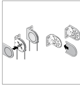
Brackets with plastic cover cap.
