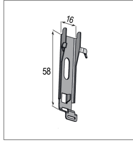
Metal clips in aluminium.
